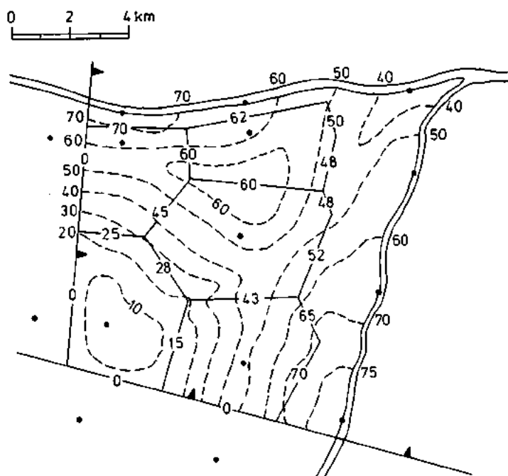
Fig. 5.4 Network superimposed on the isperm map, which shows lines of equal weighted mean hydraulic conductivity (m/d)
