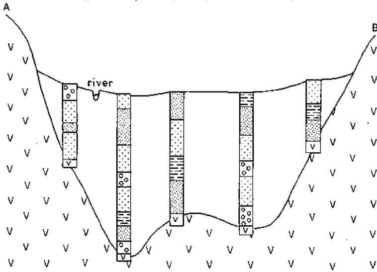
Fig. 2.7 Example of an isopach map showing the net thickness of a river-basin aquifer. The lower figure shows a cross-section of the valley
