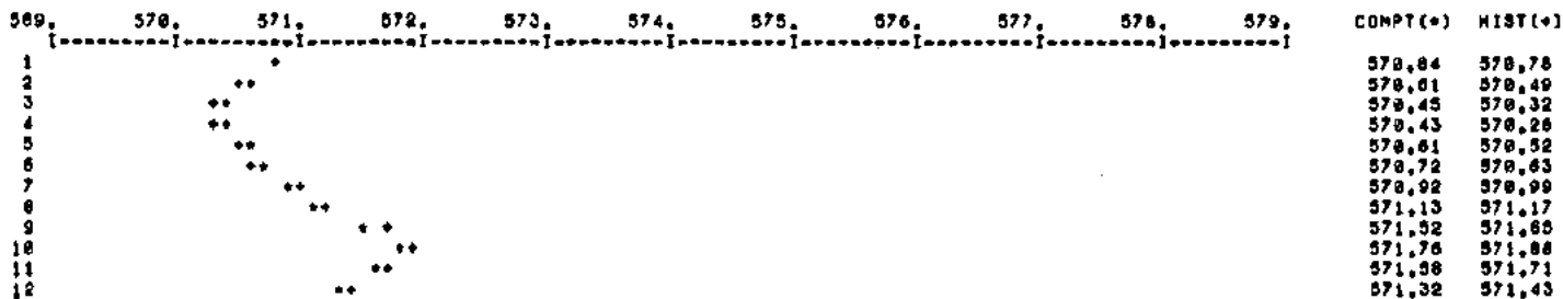
NODE NO 4 ELEVATIONS(METRES ABOVE SEALEVEL) VS, TIME( MONTH ); SURFACE ELEVATION = 581.
