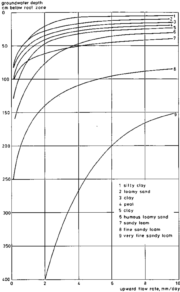
Fig. 2.3) Contribution of groundwater to the root zone in mm/d for different depths of the watertable below the root zone and for different soil types under moist conditions (soil water tension of root zone approximately 0.5 atm.) (after Doorenbos and Pruitt 1977)
