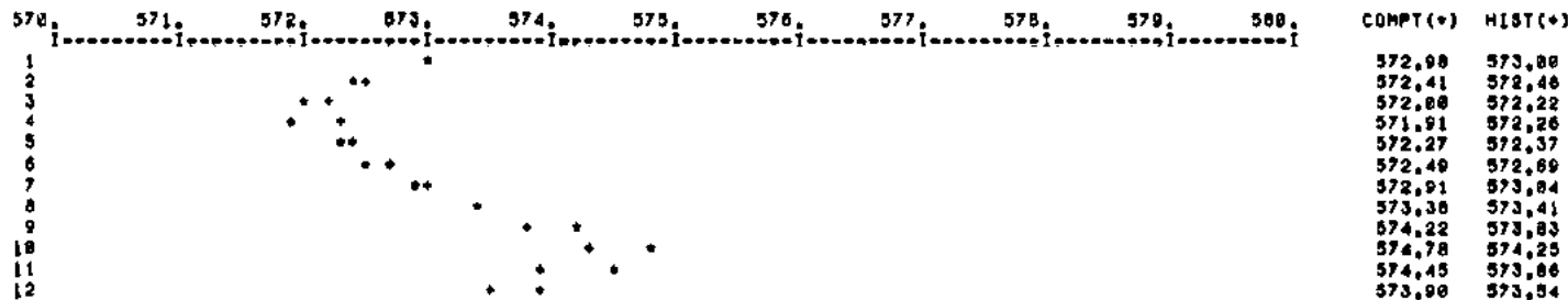
NODE NO 5 ELEVATIONS(METRES ABOVE SEALEVEL) VS, TIME( MONTH ); SURFACE ELEVATION = 583.
