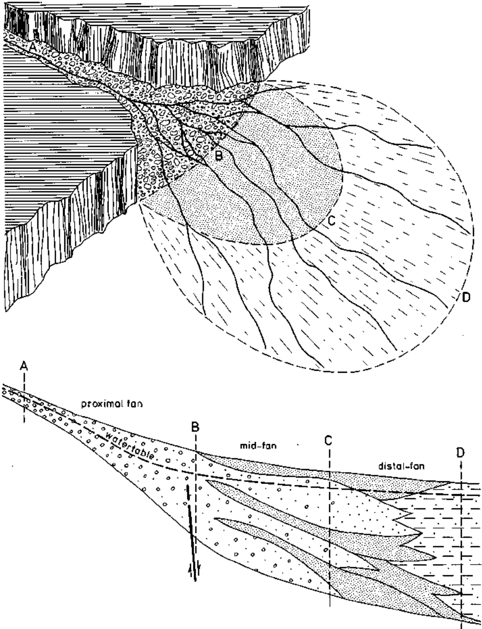
Fig. 2.12 Example of an alluvial fan and cross-section, with braided channels in the proximal part. Percolation in the proximal part enters the mid-fan at B as underflow.
